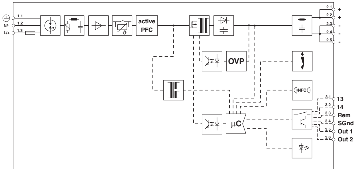
Block diagram
